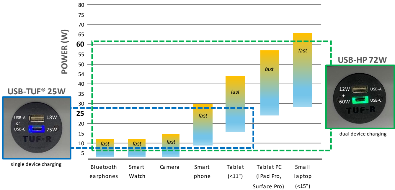
Typical power consumption of common portable devices
